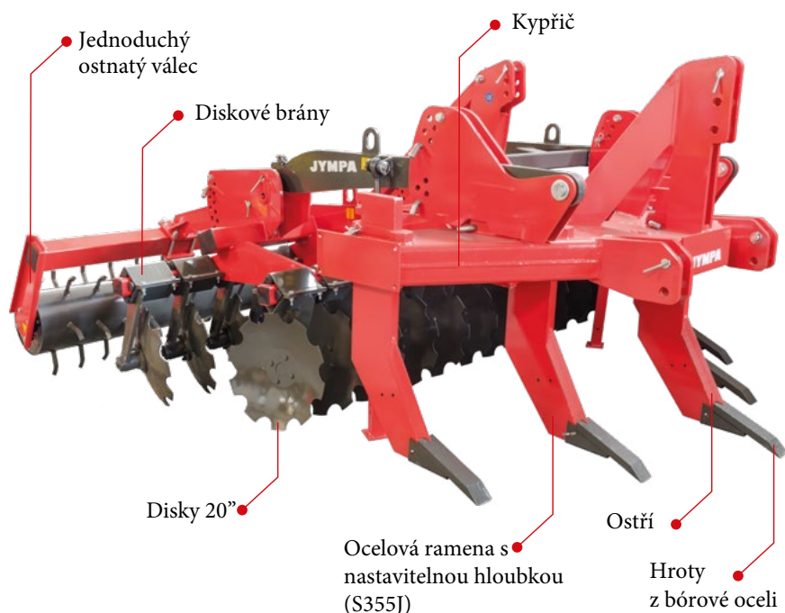
Model TANDEM-3000
